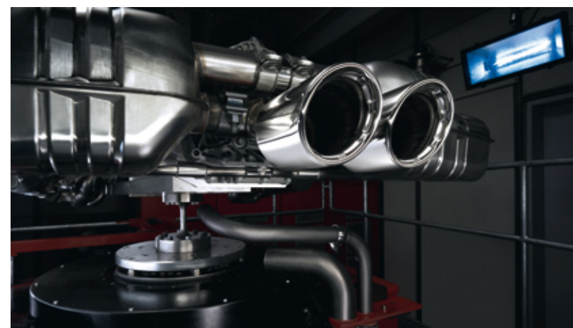
Sports tailpipe on the hot-shaker test rig in Weissach
